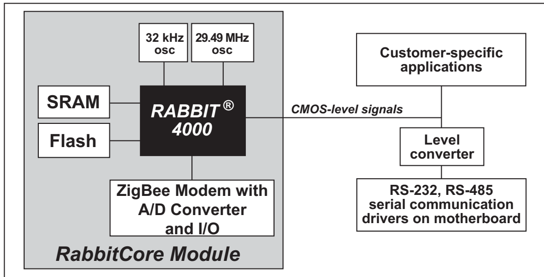
Figure 6. RCM4510W Subsystems
