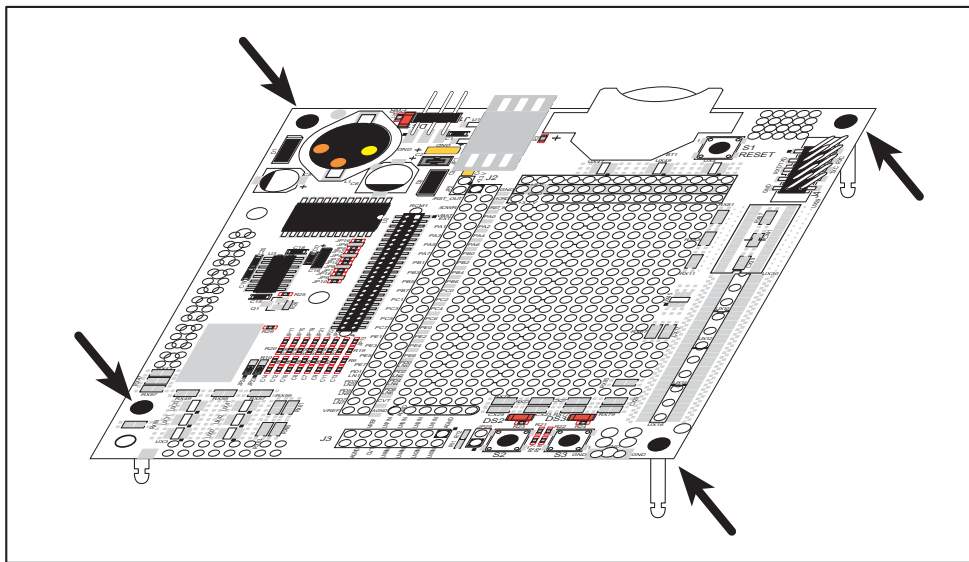
Figure 3. Insert Standoffs
